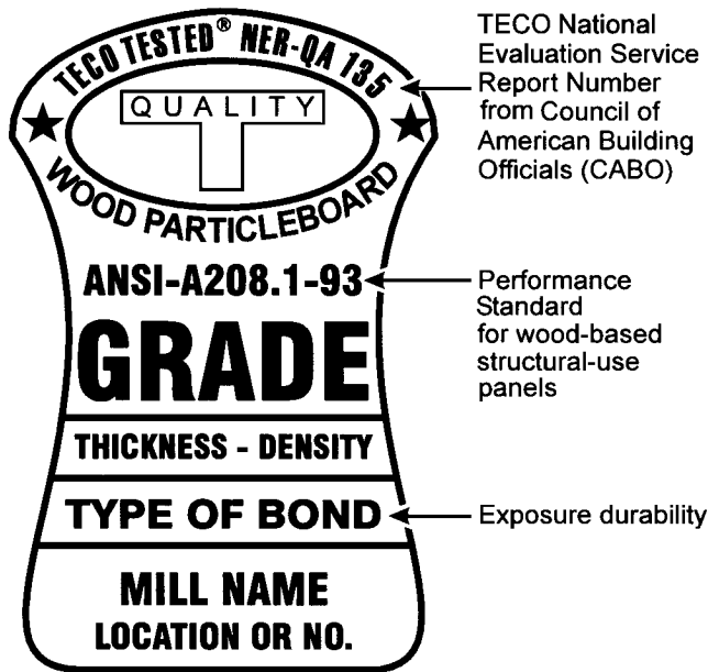
Figure 10–8. Examples of grade stamps for particleboard.
