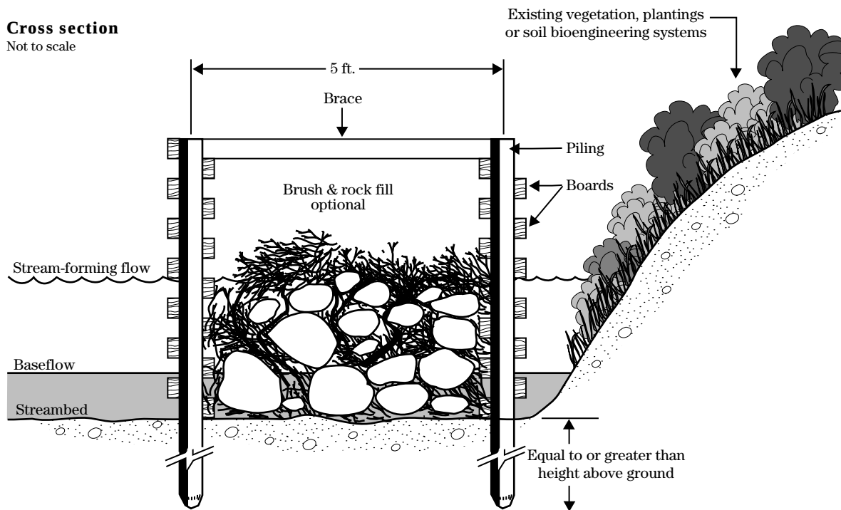
Figure 16–27 Slotted board fence details (double fence option)
