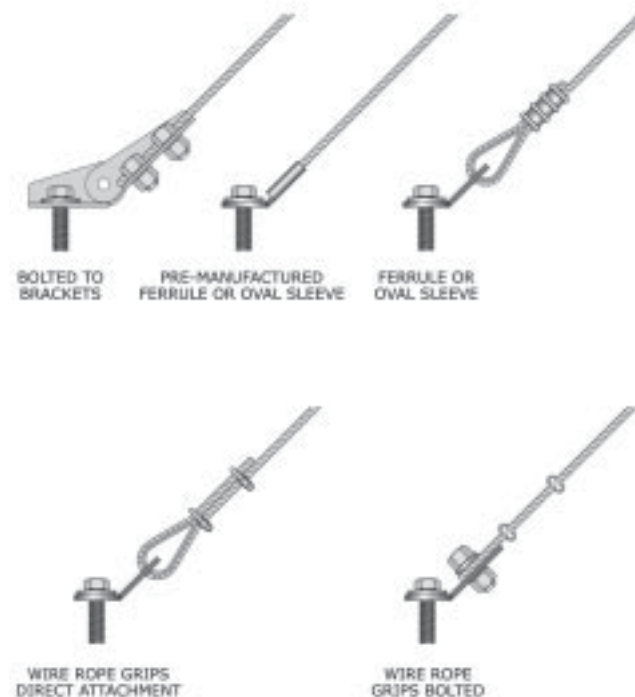
Figure 149: Cable attachments.
