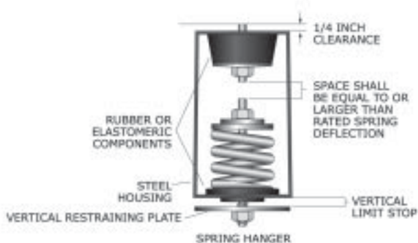
Figure 107: Isolator detail.
