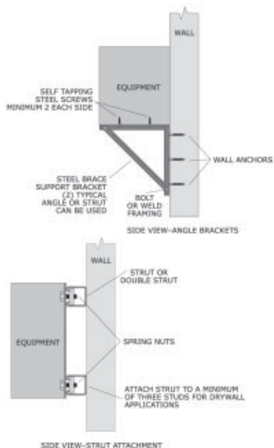
Figure 124: Angle or strut support.
