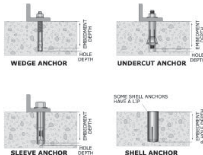
Figure 129: Embedment depth and hole depth of four anchor types.
