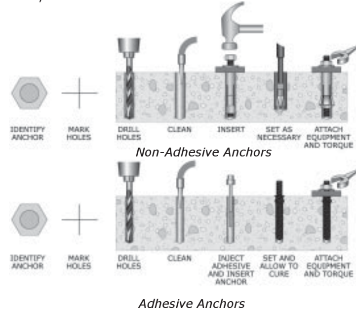
Figure 128: Summary of installation steps.
