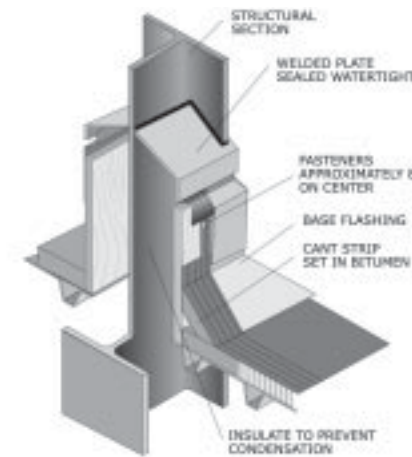
Figure 88: Flashing around a stanchion.
