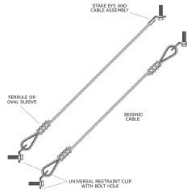
Figure 151: Ferrule assemblies.
