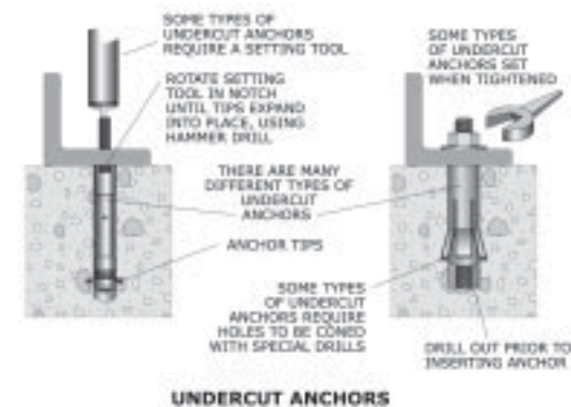
Figure 133: Set undercut anchors.
