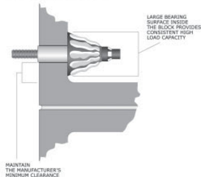
Figure 142: Umbrella anchor in a hollow block wall.
