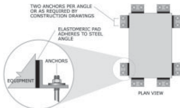
Figure 82: Equipment installed with bumpers.
