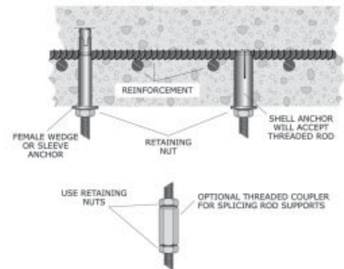
Figure 98: Concrete slab construction.
