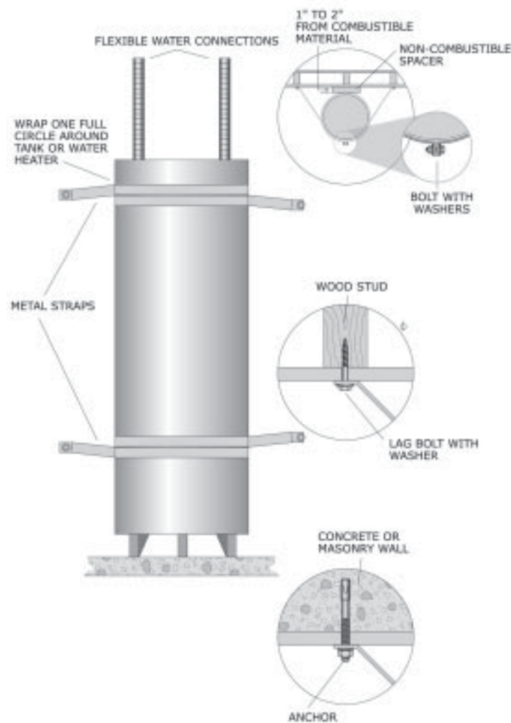
Figure 125: Electric water heater attachment.
