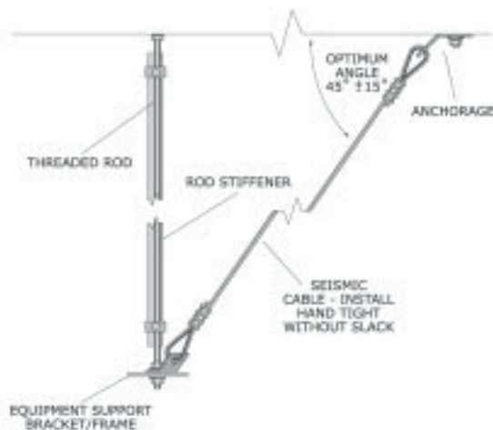
Figure 101: Attachment of cable to the equipment.
