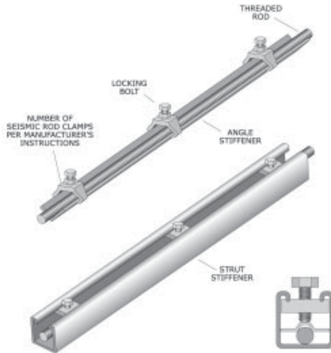
Figure 99: Rod stiffeners.
