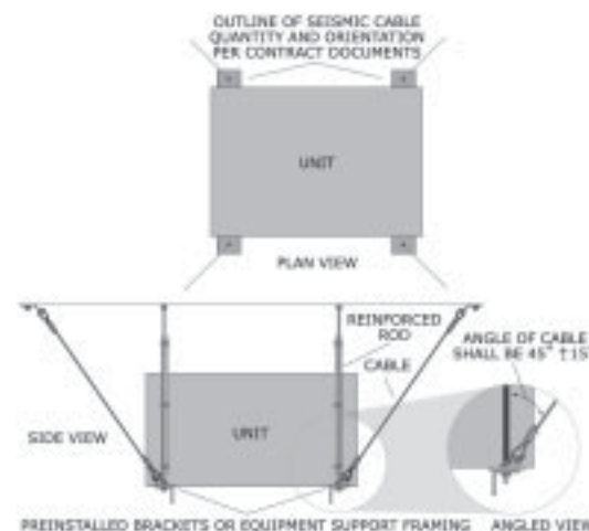
Figure 92: Rigid connection to the building structure.
