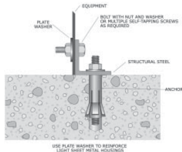
Figure 145: Bolting equipment to an angle.
