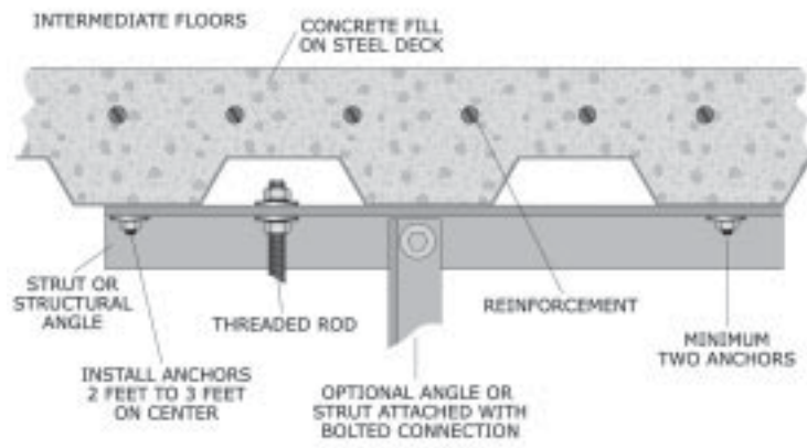
Figure 93: Cast-in-place anchor; concrete fill on steel deck.
