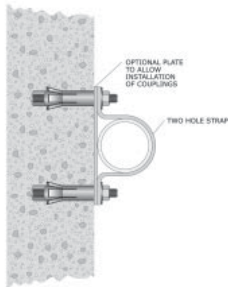
Figure 61: Direct attachment
