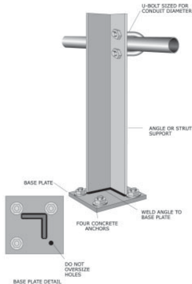
Figure 58: Single vertical support.
