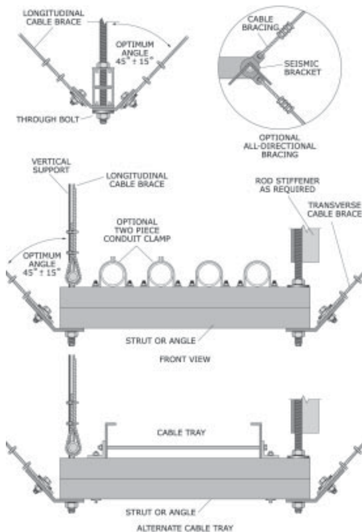
Figure 71: Trapeze support with cable lateral supports.
