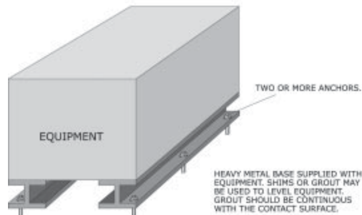
Figure 75: Direct attachment of equipment with structural steel frame or base to a building.
