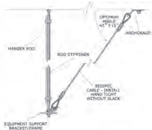
Figure 103: Attachment of cable to the equipment.
