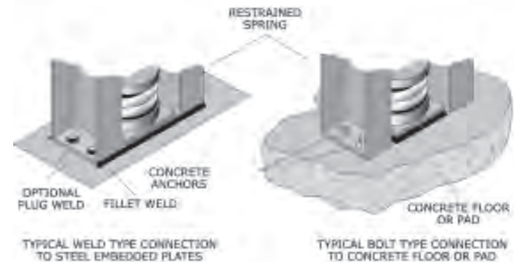
Figure 118: Attachment of restrained springs to the building structure.
