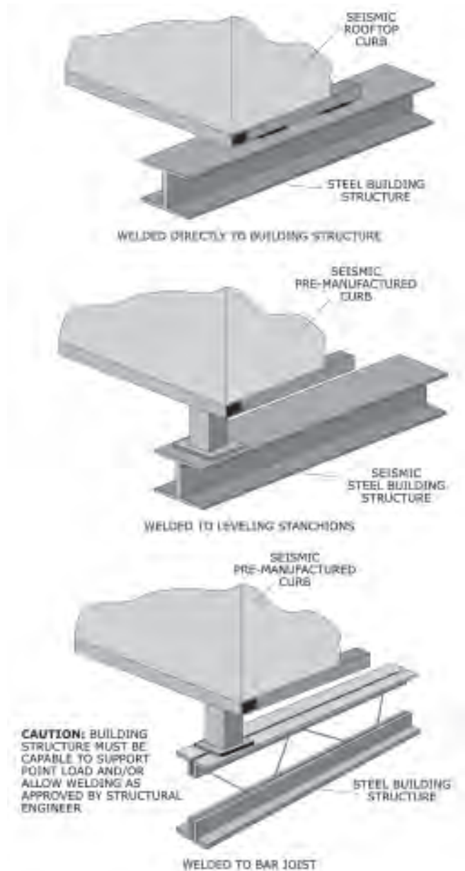
Figure 89: Pre-manufactured curb attached to the building structure.
