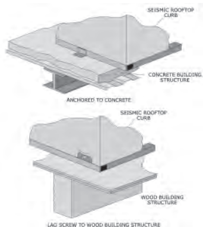
Figure 88: Pre-manufactured curb attached to a roof.
