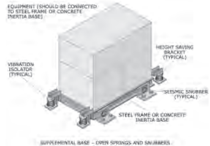
Figure 120: Typical installation of open springs and snubbers.
