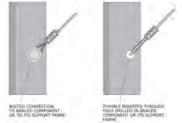
Figure 154: Ferrule attachments.
