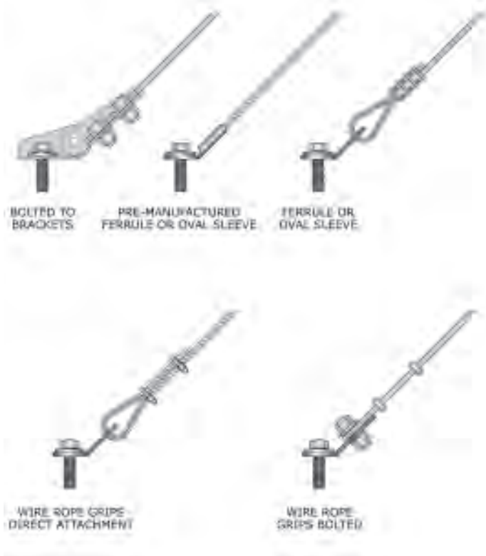
Figure 151: Cable attachments
