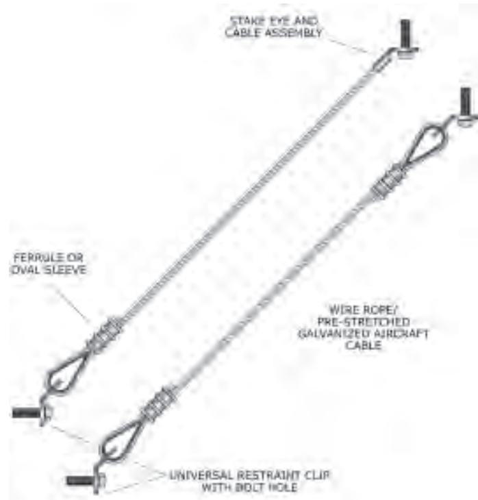
Figure 153: Ferrule assemblies.
