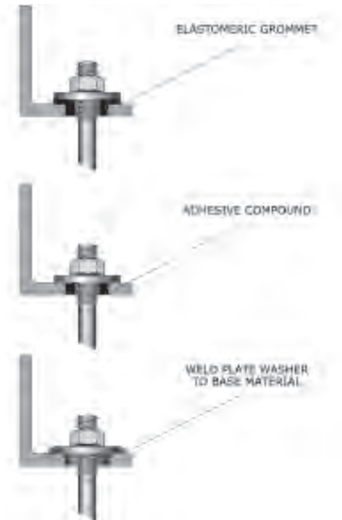
Figure 71: Three options to repair oversized holes.
