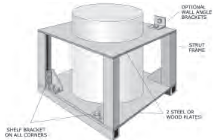
Figure 83: Tank and gas cylinder support.
