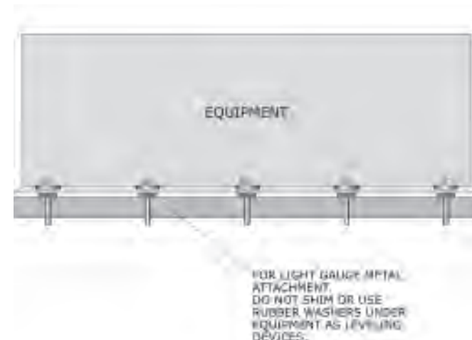
Figure 69: Side view of equipment with sheet steel housing.
