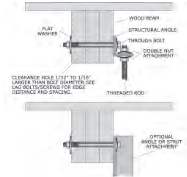
Figure 97: Wood beam construction.
