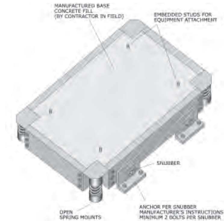
Figure 122: Concrete-filled inertia base.
