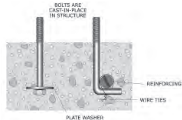
Figure 139: Bolting equipment to cast-in-place anchors.
