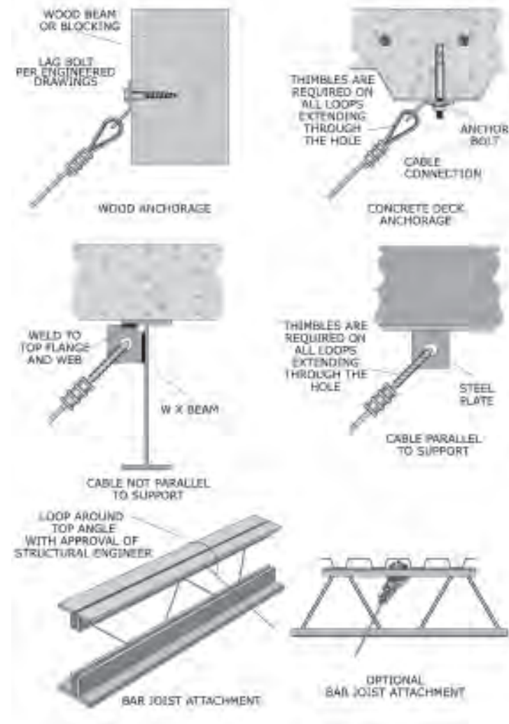
Figure 102: Attachment of cable to the building structure.
