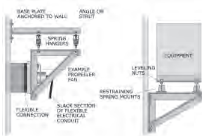
Figure 128: Wall-mounted, vibration-isolated equipment.
