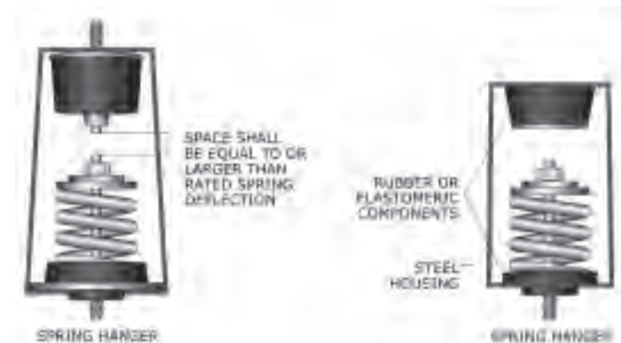
Figure 109: Isolator detail.
