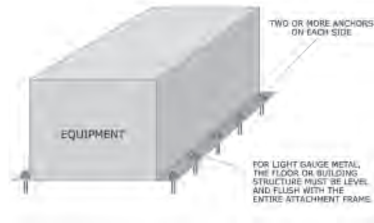
Figure 68: Direct attachment of equipment with sheet steel housing to a building.
