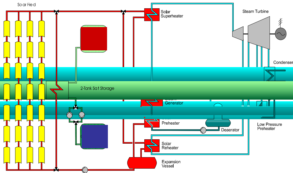
Figure 4: Parabolic trough system schematic
