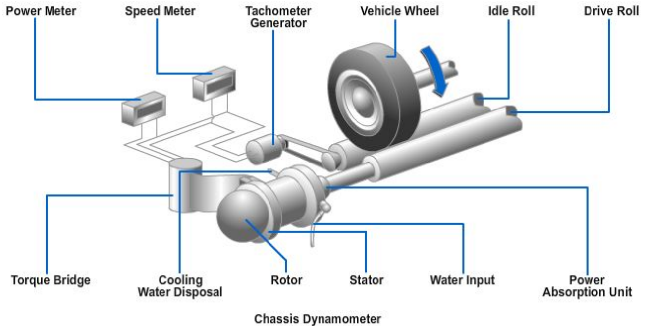
Figure 2-15 — Chassis dynamometer.
