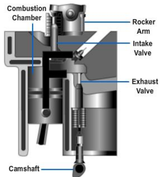
Figure 2-21 – F-Head engine.
