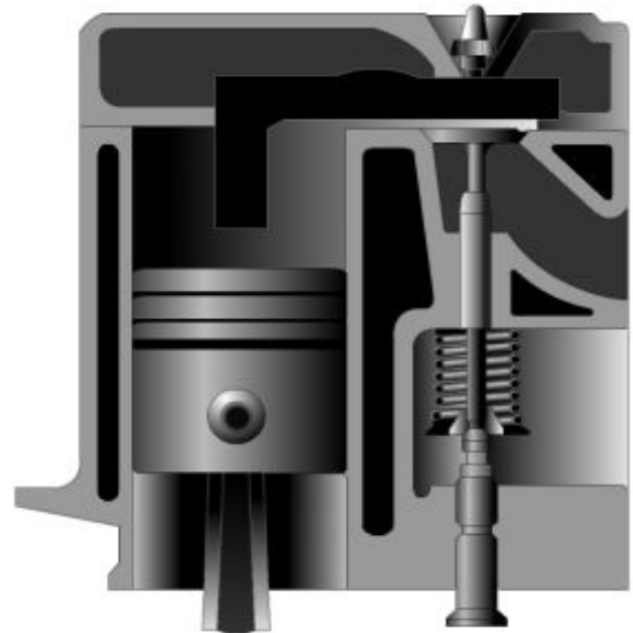
Figure 2-19– L-Head engine.
