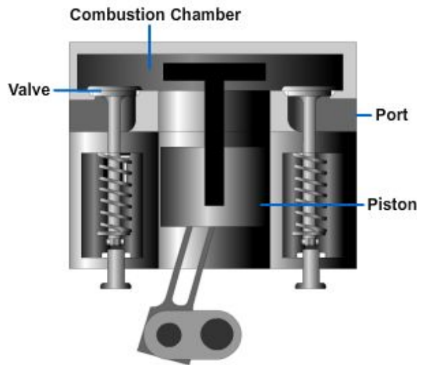
Figure 2-22 – T-Head engine.
