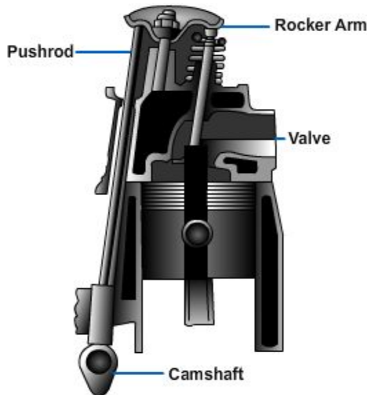
Figure 2-20 – I-Head engine.
