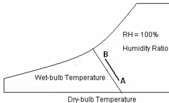
Psychrometric chart of Direct Evaporative Cooling
