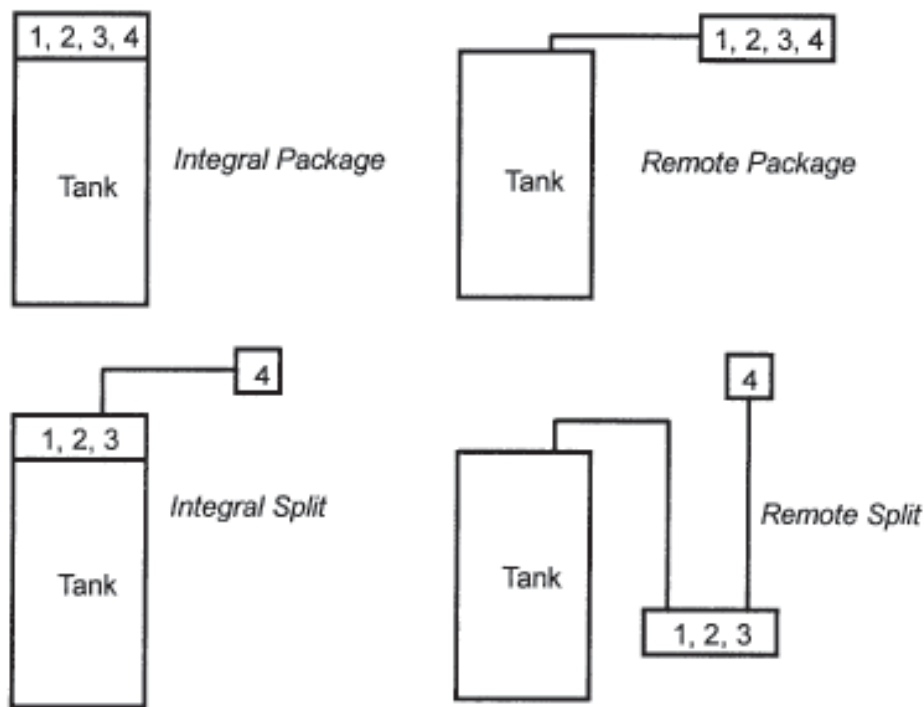
Figure 2. HPWH Configurations Found in the Market
