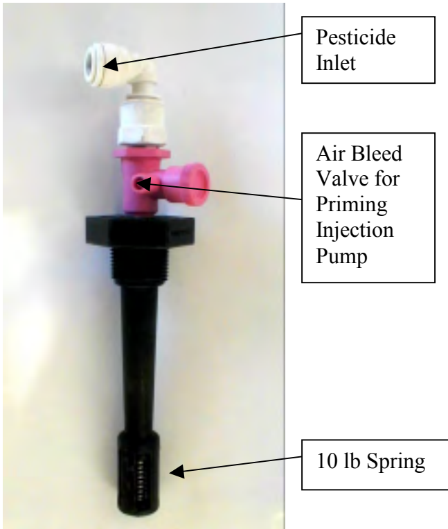
Figure 9: Injection quill with check valve
