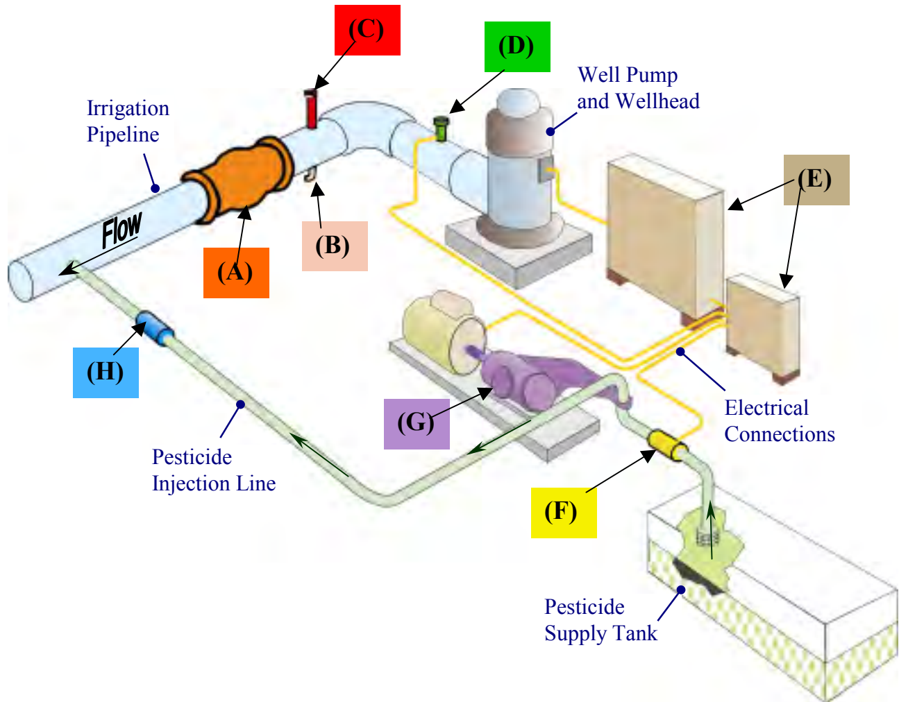
Figure 5: Schematic of a pesticide injection system with the eight required items.
