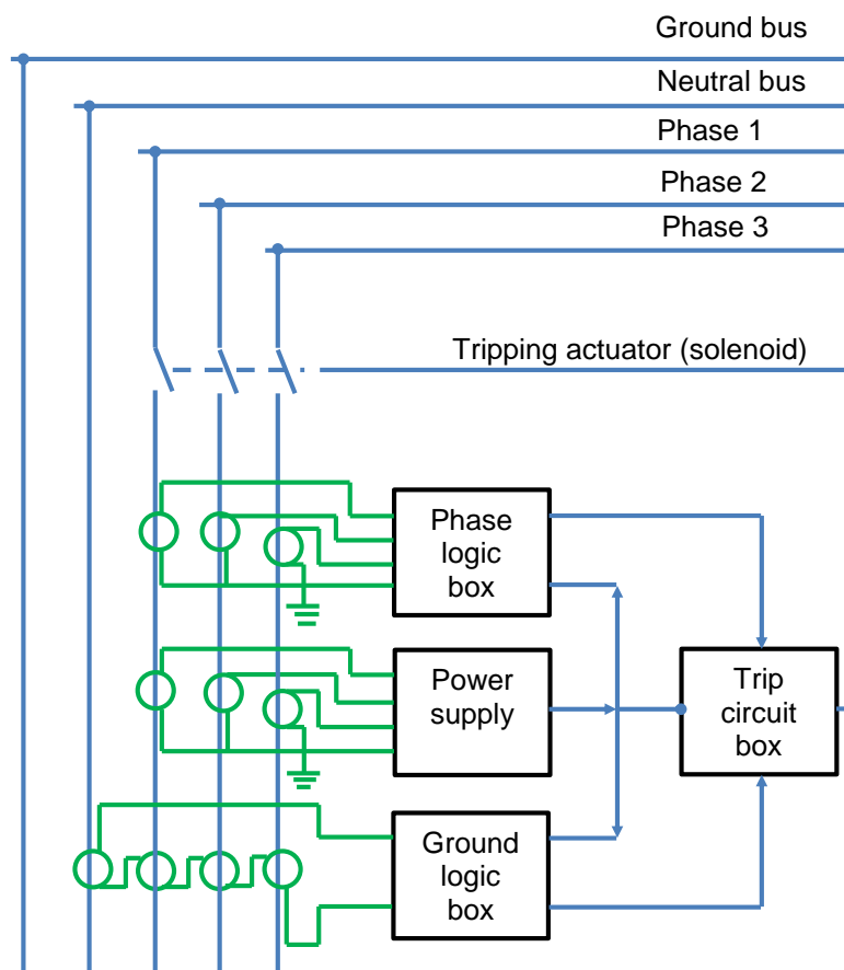
Figure 1. Functional scheme of static-trip element
