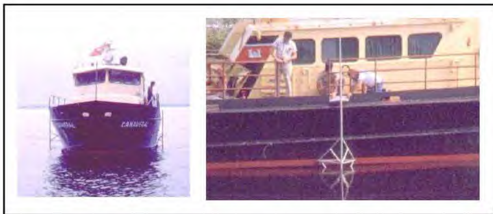
Figure 5-10. Raytheon 719 CSS three-channel hull mounted sweep ca 1970s. (Jacksonville District)
