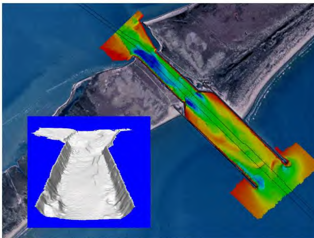
Figure 6-5. Full-coverage multibeam survey of coastal inlet navigation project and shore protection jetties. (Galveston District)
