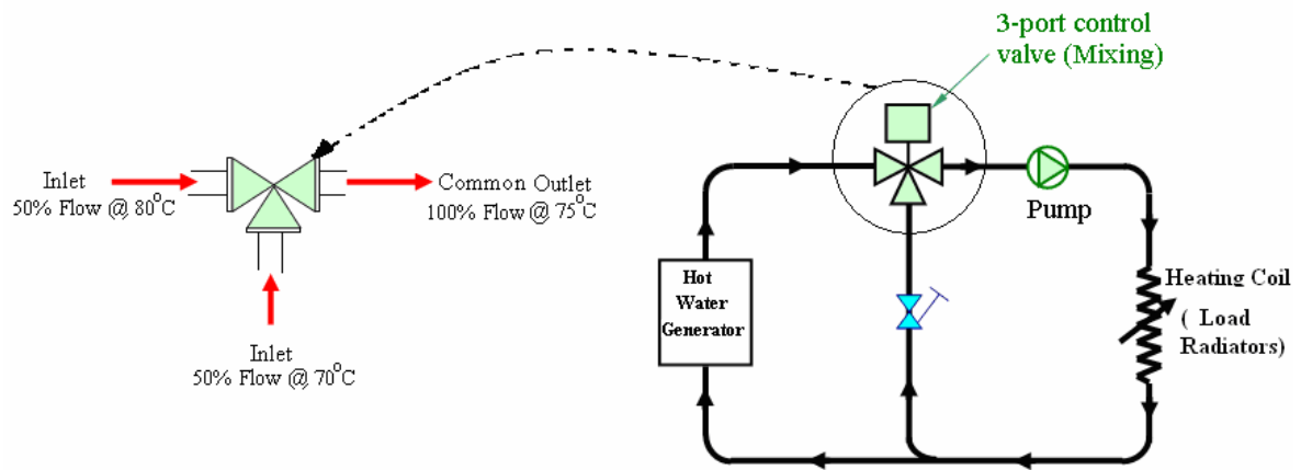
Mixing Valve in Heating Applications
