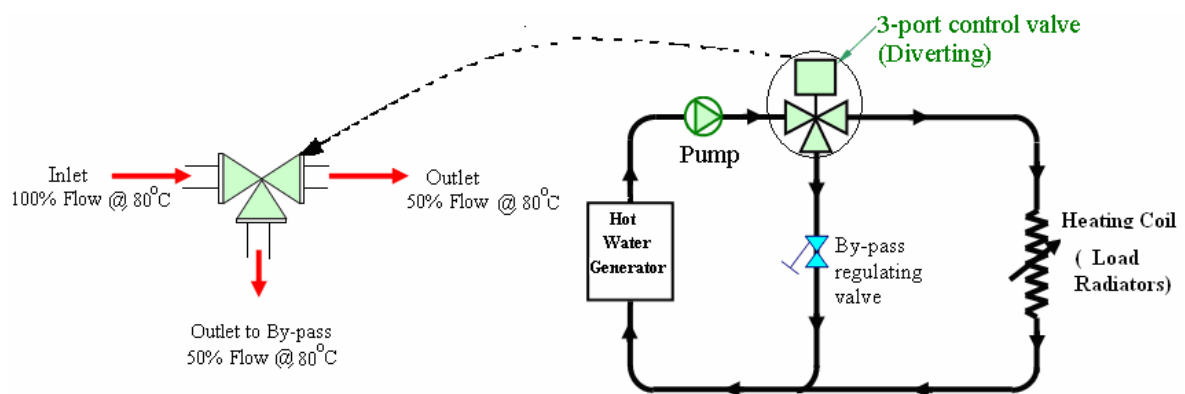
Diverting Valve in Heating Applications
