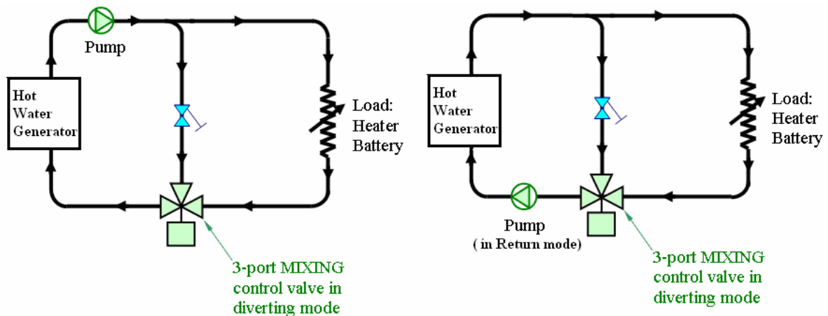
3 - Port Mixing Valve as Diverting Valve Application
