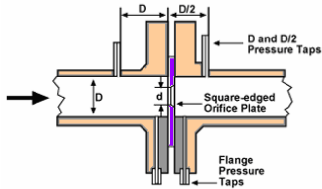
Concentric Orifice
