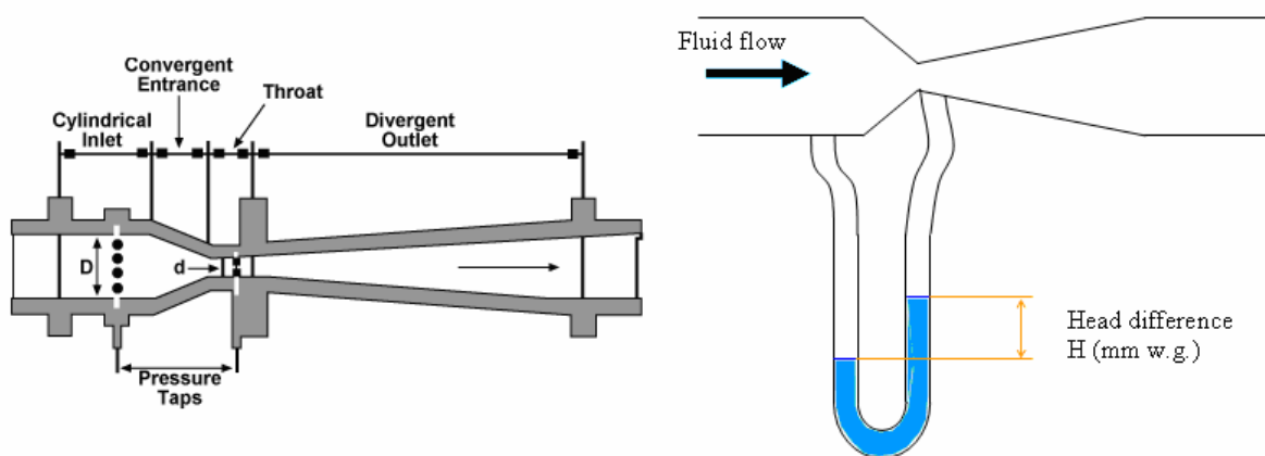
Venturi Tube Measurement
