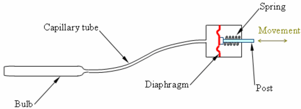
Bulb & Capillary Sensor
