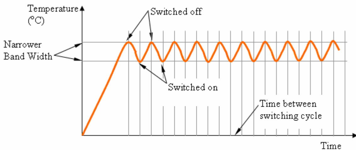
Temperature / Time Graph for Open Loop Control of Oven
