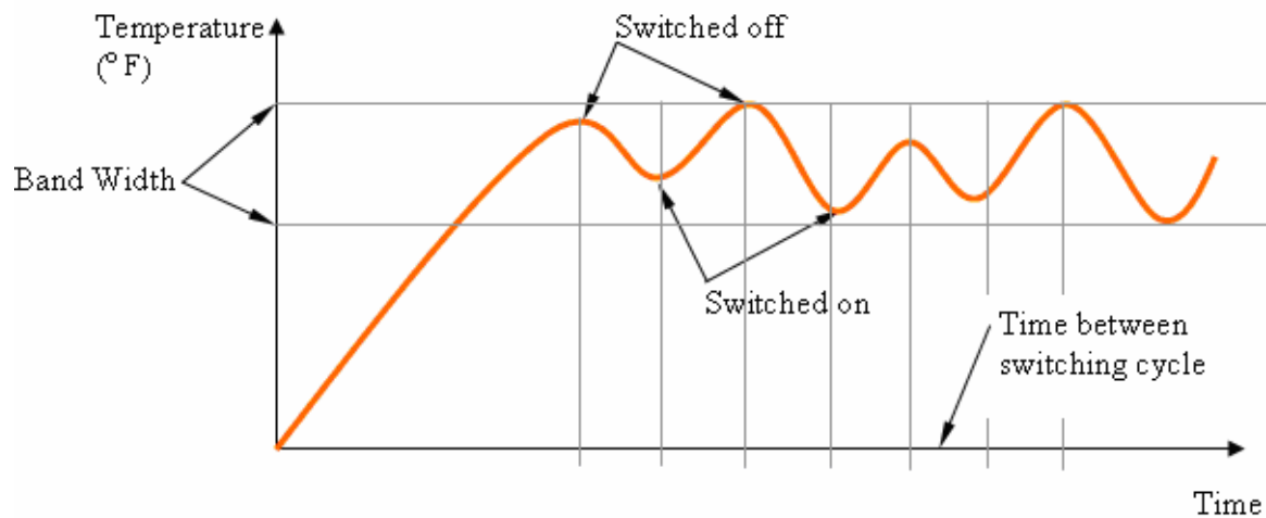
Temperature / Time Graph for Open Loop Control of Oven
