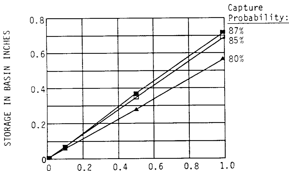
Figure B-6 Capture Volumes for a 40-hour Drain Time and Several Runoff Event Capture Probabilities (Urbonas et al., 1990) (Reprinted with permission from ASCE)
