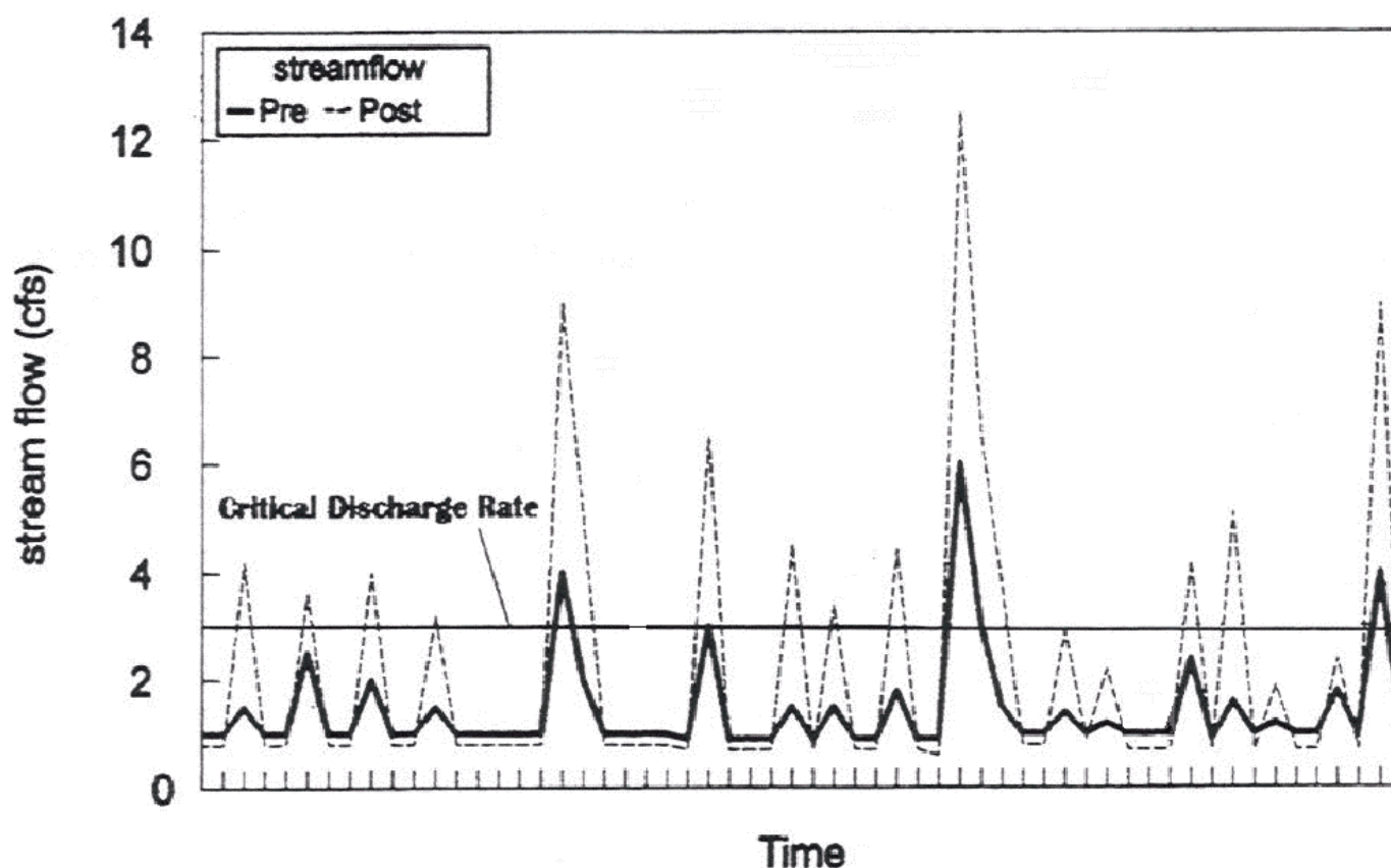
Figure 2-5 Depiction of Increased Frequency of Flows Greater Than the Critical Discharge Rate in a Stream after Development (modified after MDE, 2000)
