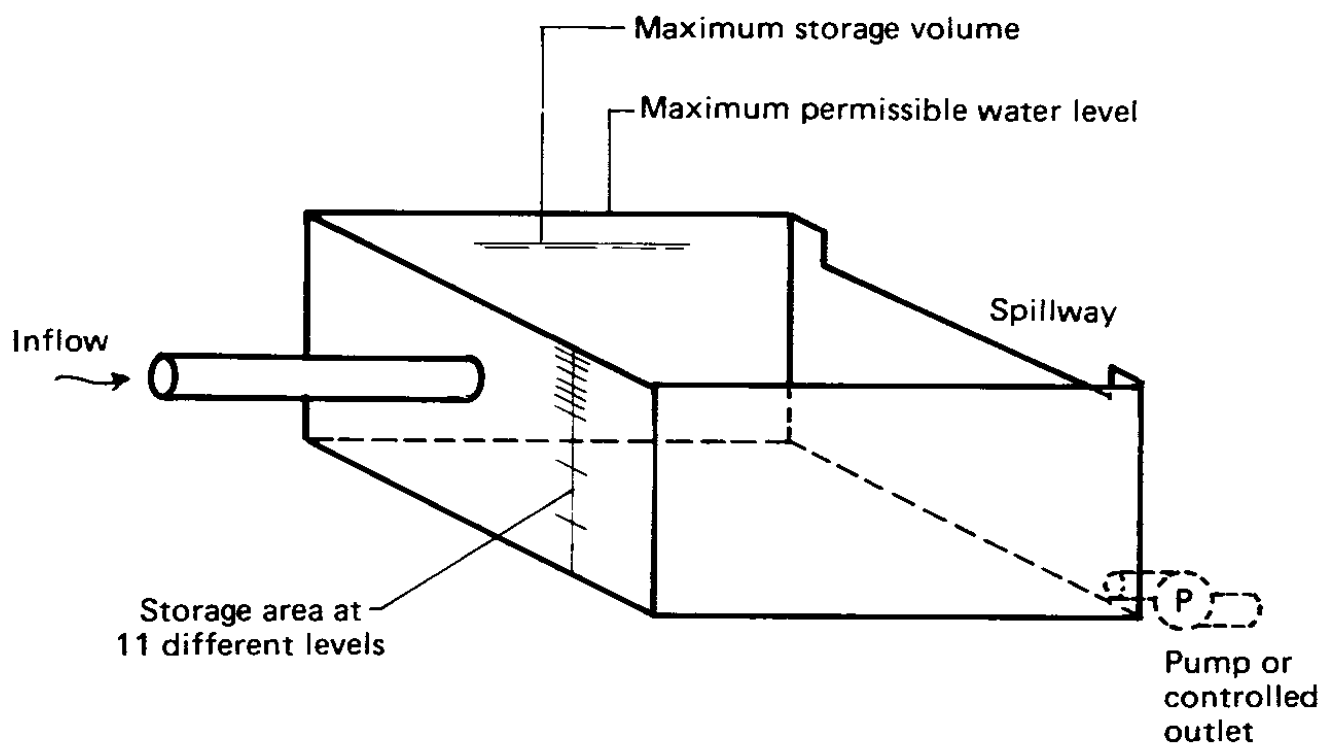
Figure A-2 Detention facility as defined in Transport Block
