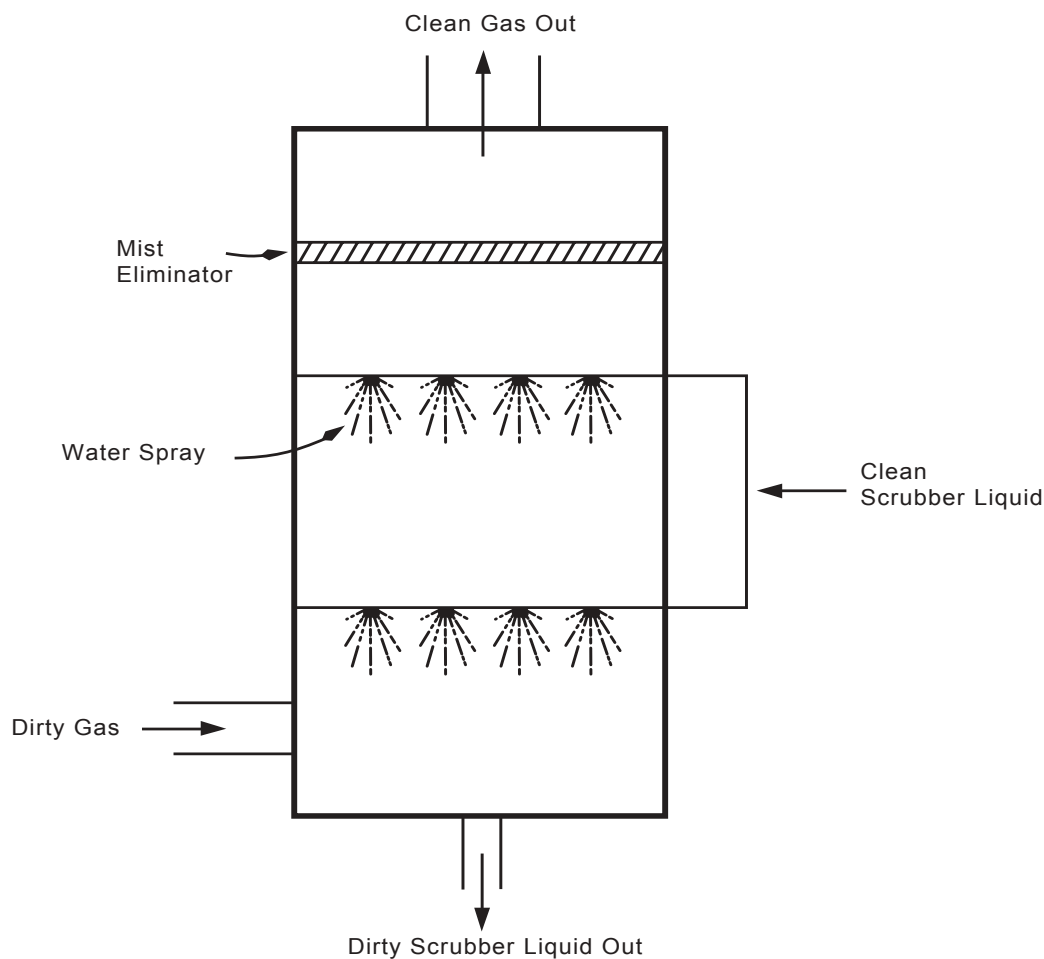
Figure 2.1: Spray Tower [4]
