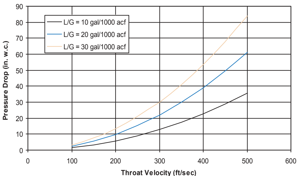
Figure 2.10: Relationship between Pressure Drop, Throat Velocity and L/G
