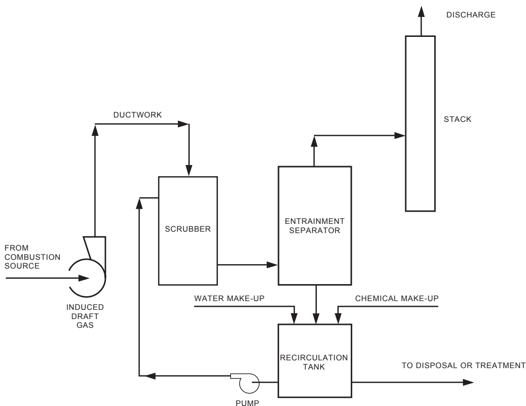
Figure 2.4: Schematic of Venturi Scrubber System
