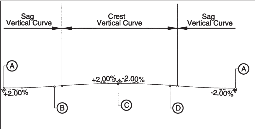
Exhibit 6-36. Sample central island profile.
