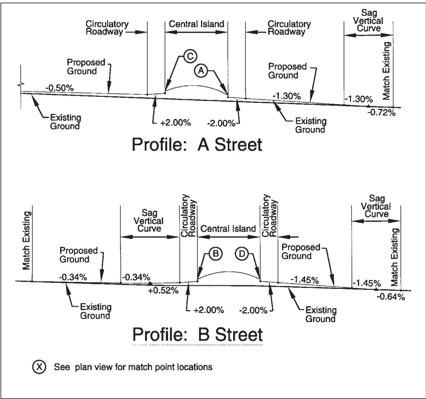
Exhibit 6-35. Sample approach profile.
