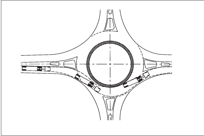
Exhibit 6-15. Through-movement swept path of WB-15 (WB-50) vehicle.
