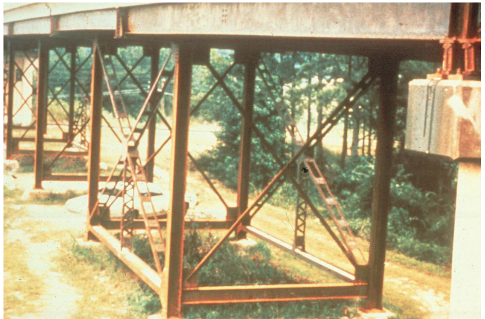
Figure P.1.75 Column Bent
