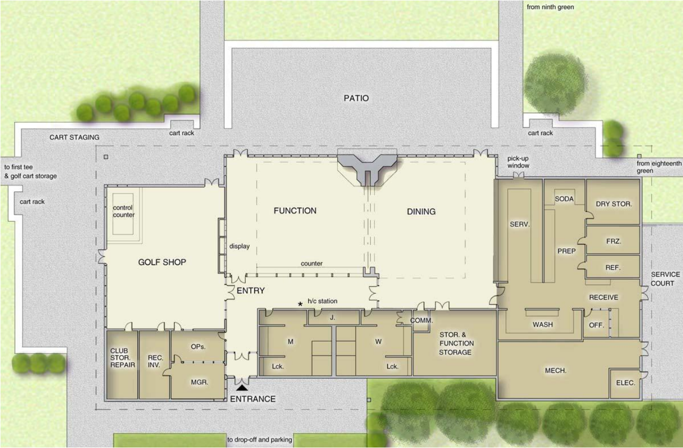
Figure 13 Example Plan – Medium Clubhouse
