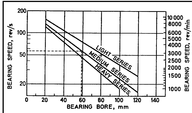
Figure 10-3. Approximate maximum speeds for grease-lubricated bearings ((Reference: Neale, M. J., Lubrication: A Tribology Handbook. Butterworth-Heinemann Ltd, Oxford, England)
