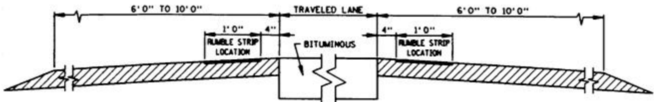
SECTION VIEW OF TWO-LANE ROADWAY - Types 2 or 3 (WITH 6' 0" TO 10' 0" PAVED SHOULDERS)
