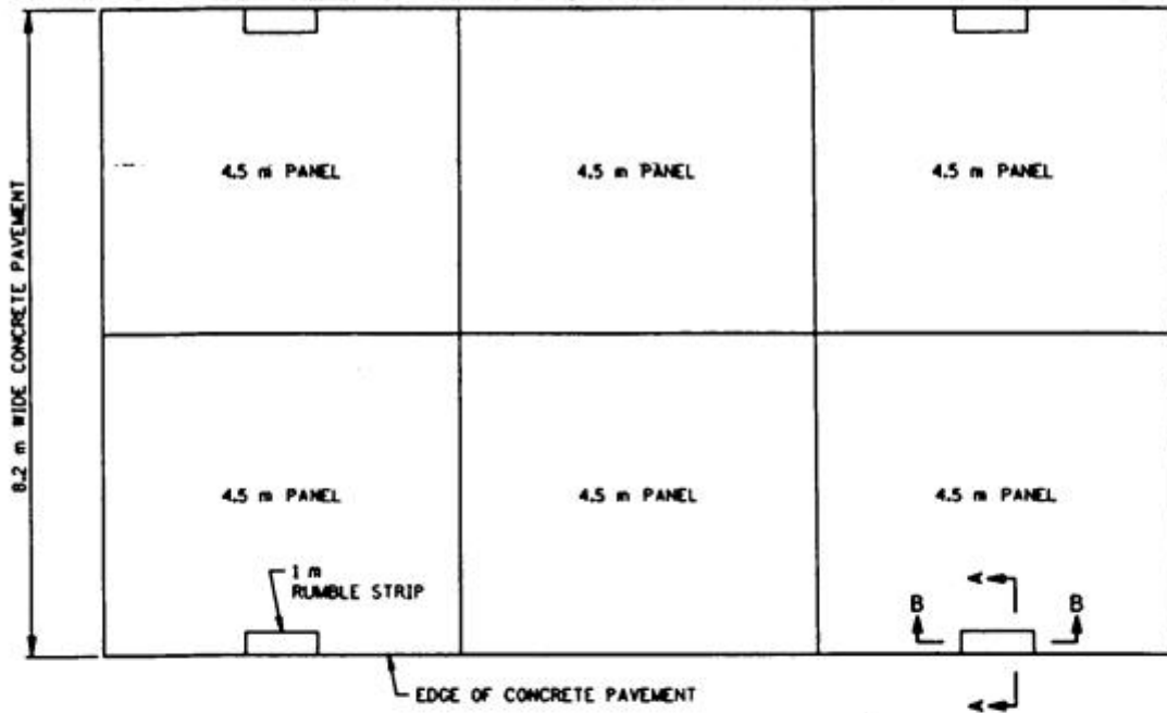
PLAN VIEW - Type 4
