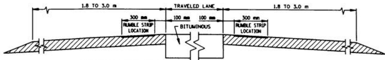
SECTION VIEW OF TWO-LANE ROADWAY - Types 2 or 3 (WITH 1.8 TO 3.0 m PAVED SHOULDERS)
