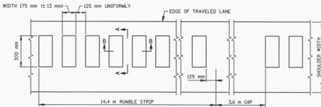
PLAN VIEW B - Type 2 INTERMITTENT PATTERN
