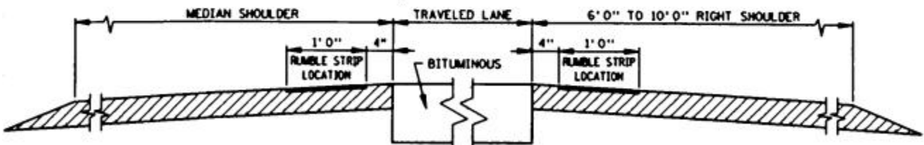
SECTION VIEW OF MULTI-LANE ROADWAY - Types 2 and 3 (ONE ROADWAY SHOWN)
