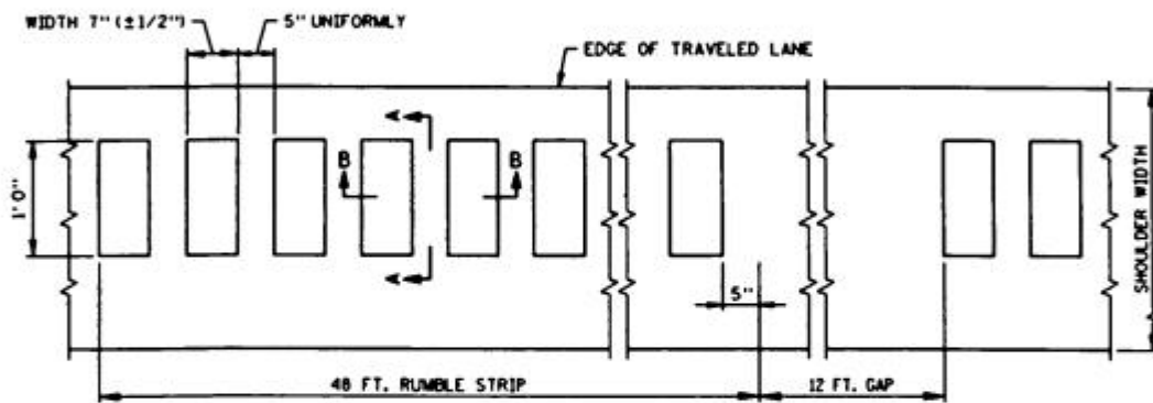
PLAN VIEW B - Type 2 INTERMITTENT PATTERN
