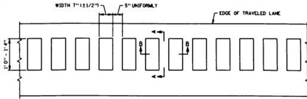
PLAN VIEW A - Types 1 and 3 CONTINUOUS
