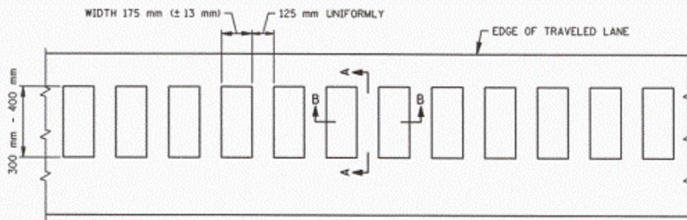
PLAN VIEW A - Types 1 and 3 CONTINUOUS
