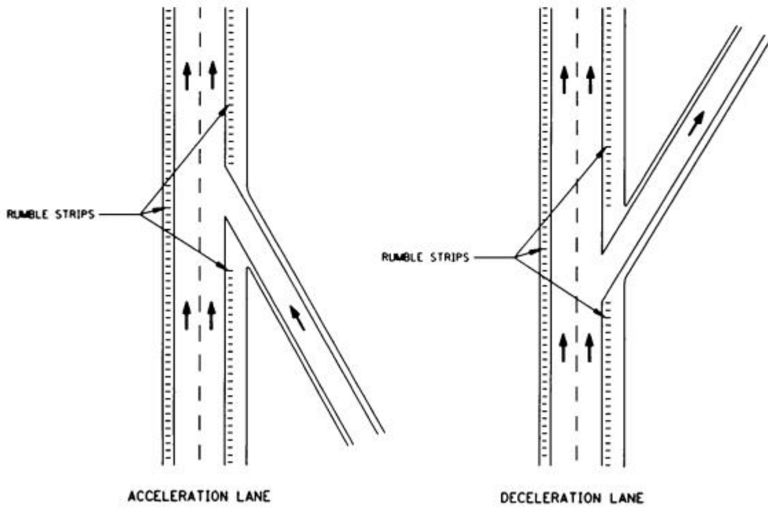
SHOULDER RUMBLE STRIP - APPROPRIATE BREAKS FIGURE 4 - ENGLISH
