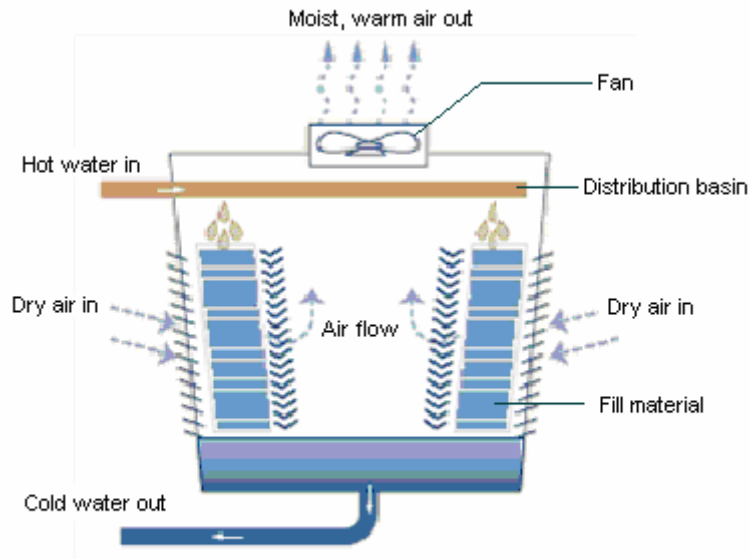
Crossflow Type Design
